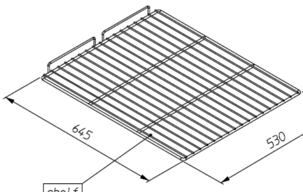
shelf 8 pcs plastic coated shelves max. load kg. 48
